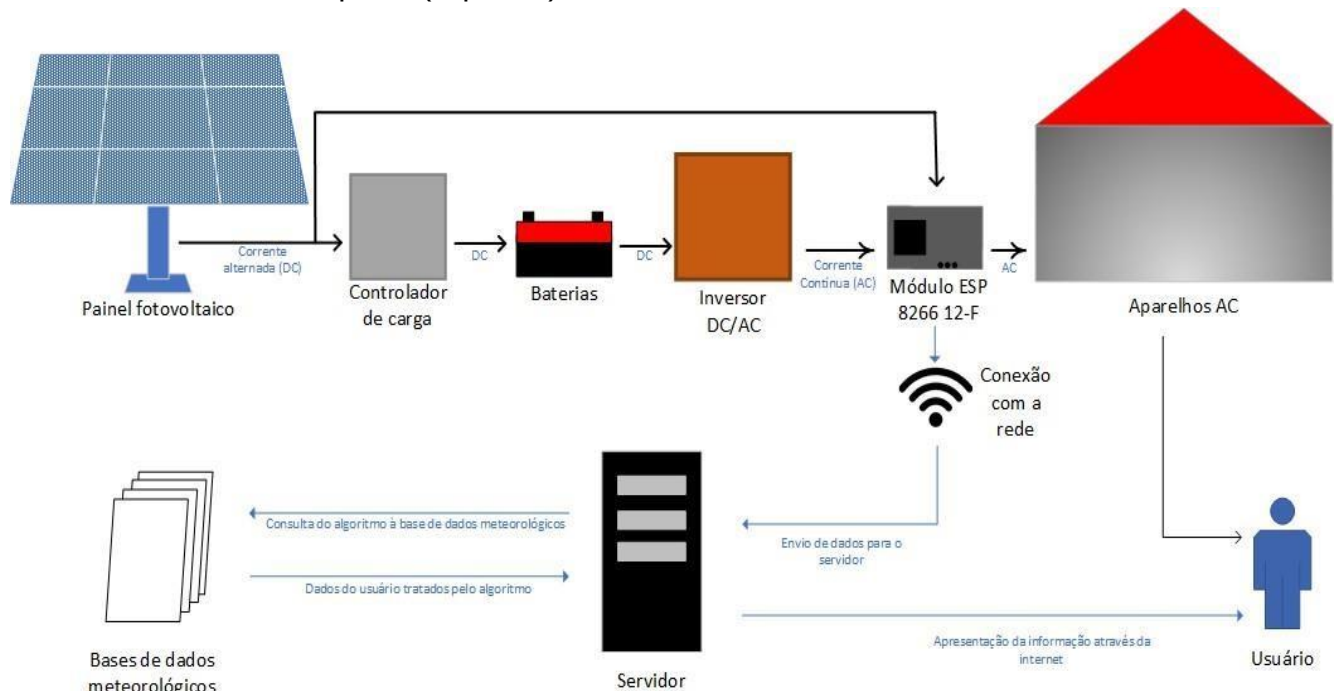
Figure 5 – Off-Grid energy acquisition model with ESP8266 implemented. Source: From the author (2020).
