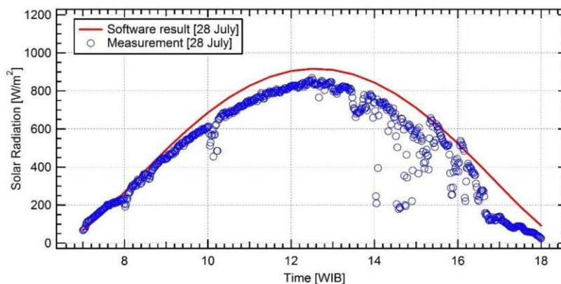
Figure 1 – Comparison between software estimates and measured values under clear-sky conditions. Source: Ambarita (2017, p. 4).
