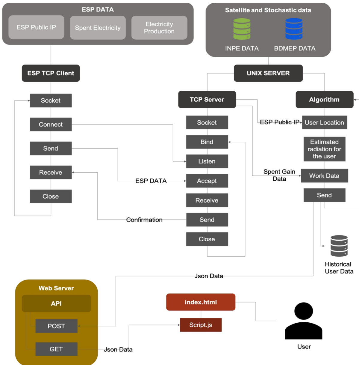
Figure 7 – Data flow. Source: Author (2021).
