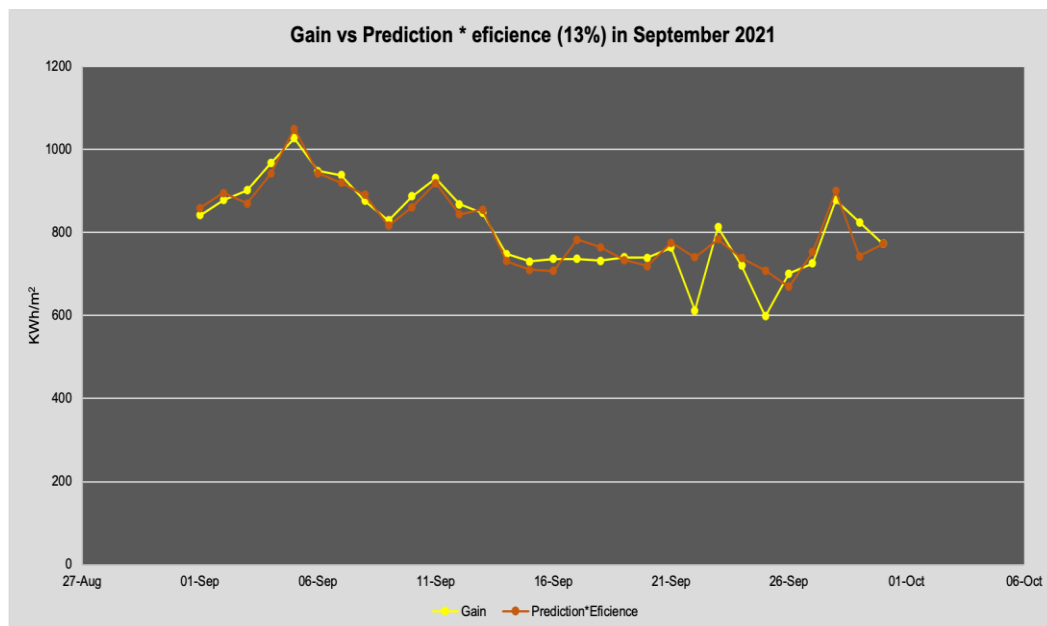
Figure 13 – Gain compared with the product of the Prediction by the efficiency of the solar panel Source: From the author (2021).
