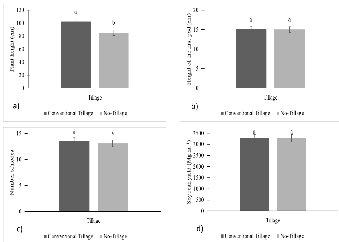
Figure 6. Plant height (a), first pod insertion height (b), number of nodes (c), and grain yield (d) as a function of conventional and no-till planting systems. The bars represent the standard deviation.
