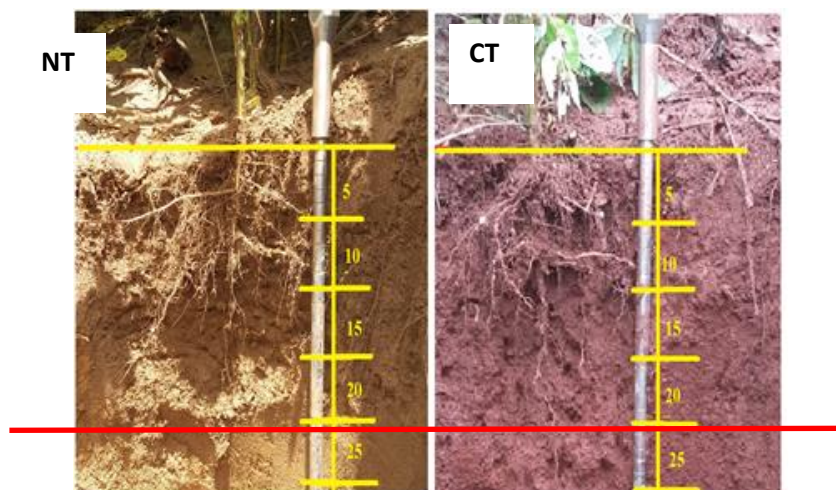
Figure 7. Root system depth (cm) of soybean plants observed in field trenches.
