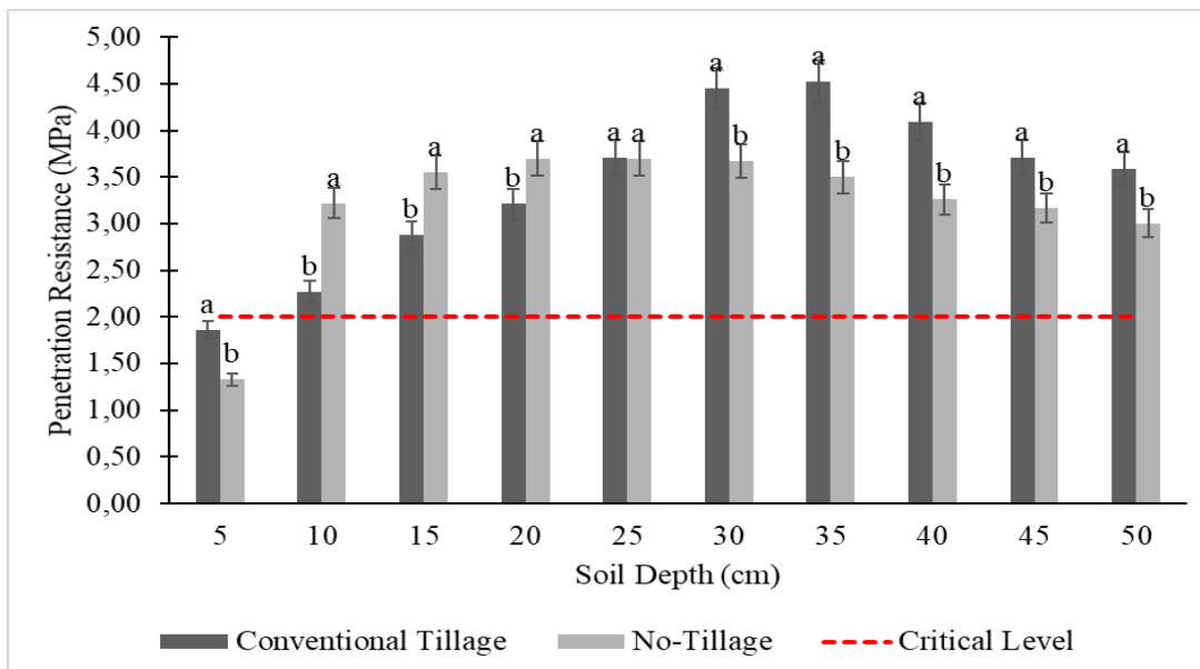
Figure 3. Penetration resistance as a function of soil depth (0–50 cm) under no-till and conventional tillage systems. The bars represent the standard deviation.
